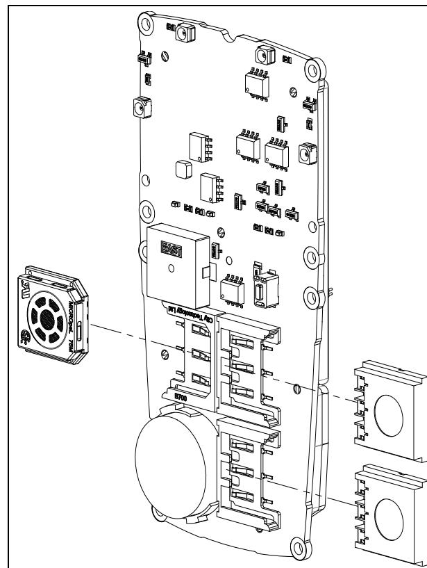
Figure 11. Sensor Positioning
